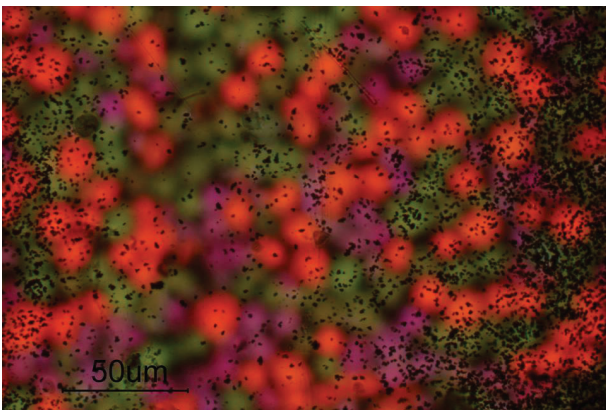
Microscopic study of the silver grain side of a Cinécolor (Autochrome) 35mm sample, ca. 1932 (HTW Berlin, 2016)
